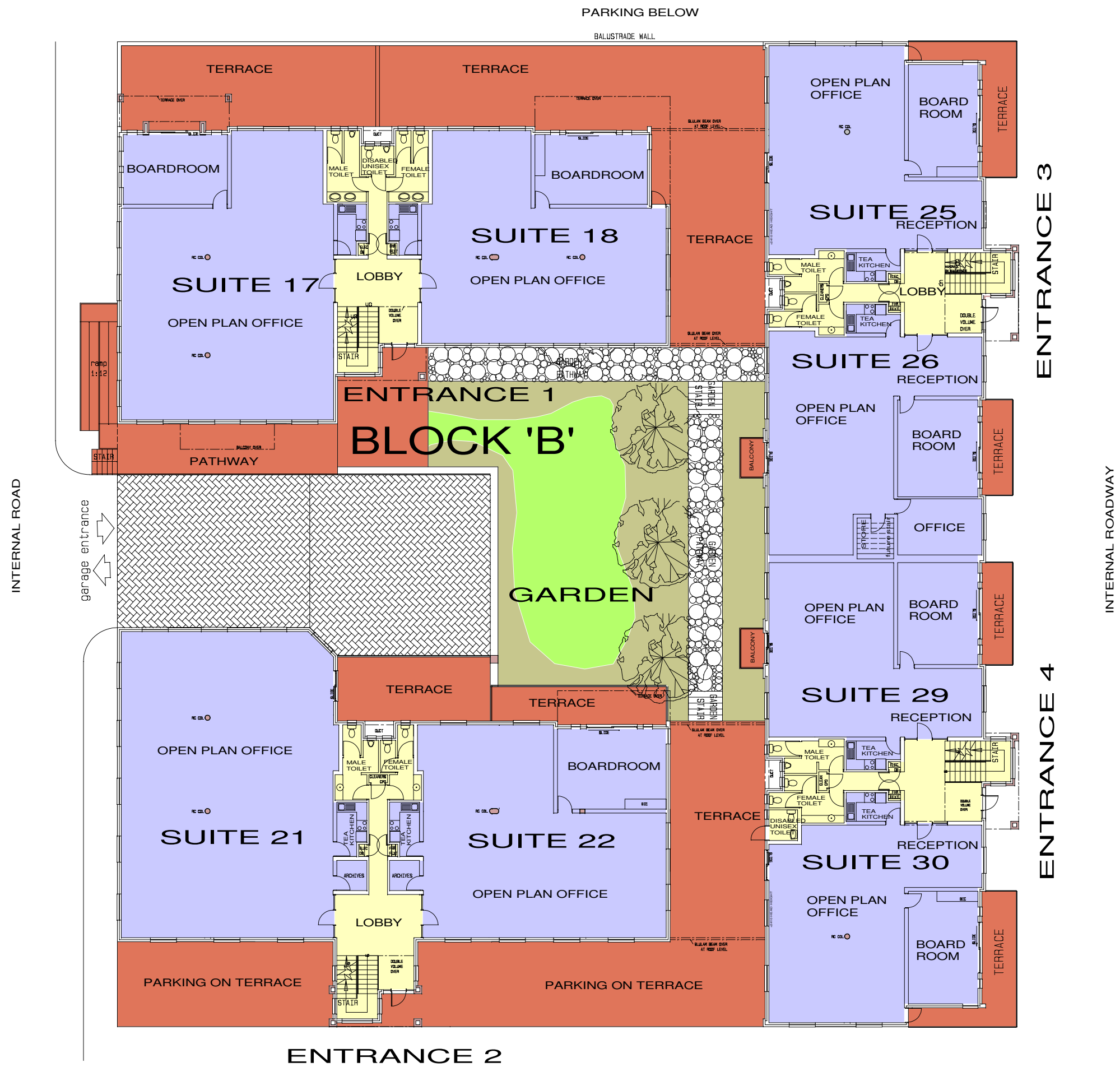
BLOCK 'B' GROUND FLOOR PLAN
