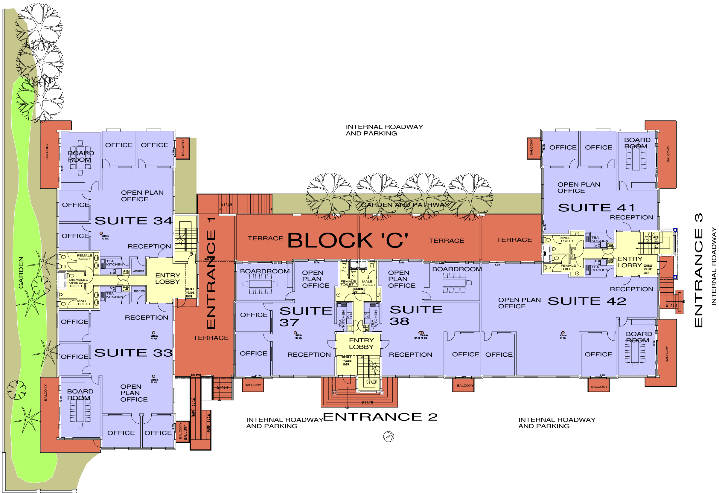
BLOCK 'C' BUILDING 2 - GROUND FLOOR PLAN
