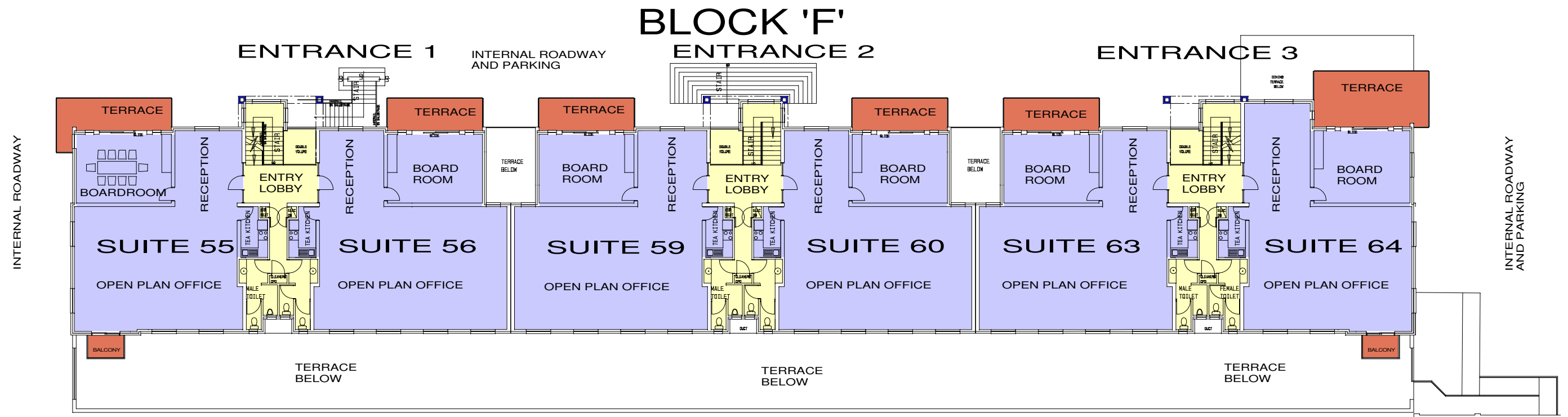
BLOCK 'F' FIRST FLOOR PLAN
